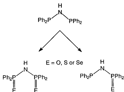
Scheme 1. Heteroatom ligands derived from DPPA.
