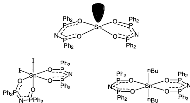
Fig. 23. The structures of [\text{Sn}(\text{Ph}_2(\text{O})\text{P})_2\text{N}]_2 , [\text{SnI}_2\{(\text{Ph}_2(\text{O})\text{P})_2\text{N}\}_2] [49] and [\text{Sn}(n\text{Bu})_2\{(\text{Ph}_2(\text{O})\text{P})_2\text{N}\}_2] [50].
