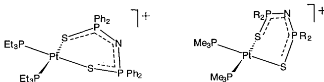
Fig. 18. The structures of [\text{Pt}\{\text{N}(\text{P}(\text{S})\text{Ph}_2)_2\}(\text{PEt}_3)_2]^+ and [\text{Pt}\{(\text{PhO})_2(\text{S})\text{PNP}(\text{S})(\text{OPh})_2\}(\text{PMe}_3)_2]^+ [43].
