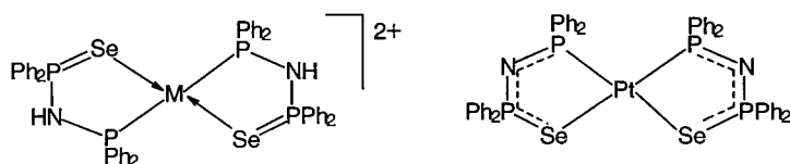
Fig. 4. The structures of [\text{Pt}\{\text{Ph}_2\text{P(Se)NHPPH}_2\}_2]\text{Cl}_2 and [\text{Pt}\{\text{Ph}_2\text{P(Se)NPPH}_2\}_2] [14].
