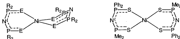
Fig. 16. The structures of [\text{Ni}\{(\text{Ph}_2(\text{S})\text{P})_2\text{N}\}_2] [6,34,35], [\text{Ni}\{(\text{Me}_2(\text{S})\text{P})_2\text{N}\}_2] [36,37], [\text{Ni}\{(\text{Pr}_2(\text{S})\text{P})_2\text{N}\}_2] [38] and [\text{Ni}\{(\text{Ph}_2(\text{S})\text{PNP}(\text{S})\text{Me}_2)\}_2] [39].
