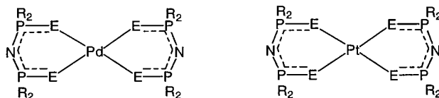
Fig. 17. The structures of [\text{Pd}(\text{PhO})_2(\text{S})\text{PNP}(\text{S})(\text{OPh})_2] [41], [\text{M}\{(\text{iPr}_2(\text{S}(\text{P})_2\text{N})_2)_2\}] ( \text{M} = \text{Pd} or \text{Pt} ) (D. Cupertino, R. Keyte, A.M.Z. Slawin, D.J. Williams, J.D. Woollins, unpublished work) and [\text{Pd}(\text{Ph}_2(\text{O})\text{PNP}(\text{Se})\text{Ph}_2)_2] ( \text{R} = \text{Ph} or \text{iPr} ) [40].
