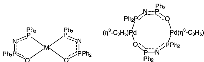
Fig. 2. The structures of \text{cis-[M}\{\text{Ph}_2\text{P(O)NPh}_2\}_2] and [\text{Pd}(\eta^3\text{-C}_3\text{H}_5)\{\text{Ph}_2\text{PNP(O)Ph}_2\}_2] [12].
